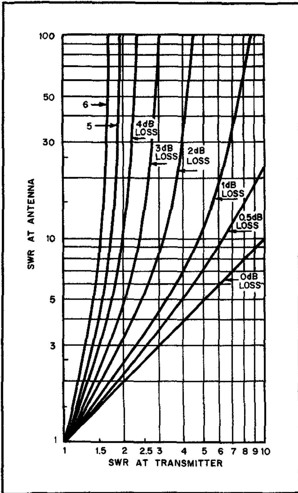
Fig. 2 — SWR at input end of transmission line vs. SWR at load end for various values of matched-line loss.
